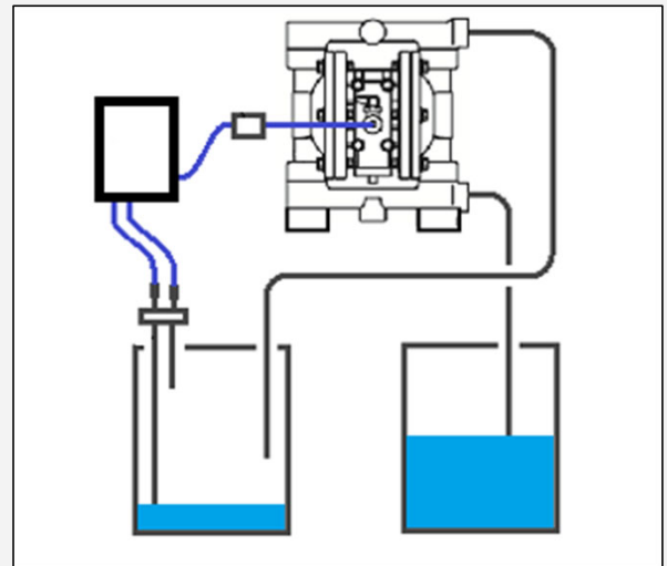
Typical System Layout
